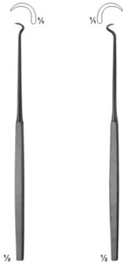
13-111 BOSE 165 mm
